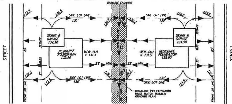
TYPICAL LOT GRADING PLAN FLOW-LINE AT REAR LOT LINE
