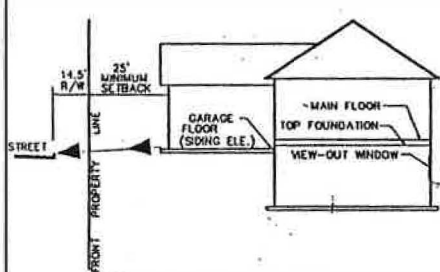
TYPICAL VIEW-OUT SECTION FLOW-LINE AT REAR LOT LINE
