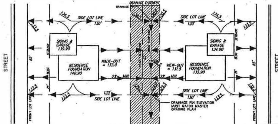
TYPICAL LOT GRADING PLAN FLOW-LINE OUTSIDE REAR LOT LINE
