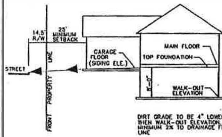
TYPICAL LOT GRADING PLAN FLOW-LINE OUTSIDE REAR LOT LINE
